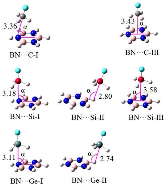
FIGURE 2 Optimized structures of the \text{BN}\cdots\text{TH}_3\text{F} ( \text{T} = \text{C}, \text{Si}, and \text{Ge} ) complexes. Distances are in Å
