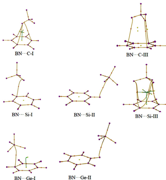
FIGURE 3 The atoms in molecules diagrams of the \sigma -hole tetrel bond complexes. Small dots refer to bond critical points
