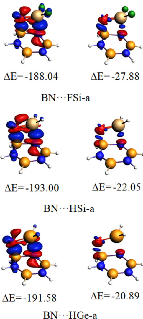
FIGURE 6 Plots of deformation densities of the pair-wise orbital interactions ( \Delta\rho ) in the a complexes of F_2SiO and H_2TO ( T = Si and Ge ) at the GGA-PBE-D3/TZ2P//MP2/aug-cc-pVTZ level. The associated orbital interaction energies are given in kcal/mol. The color code of the charge flow is red \rightarrow blue, and the isovalue for \Delta\rho is 0.005 a.u.
