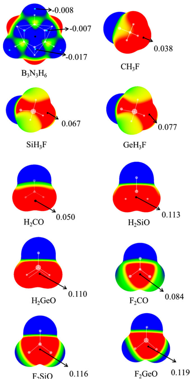
FIGURE 1 Molecular electrostatic potential diagrams of the monomers. Color ranges, in a.u., are: red, greater than 0.02; yellow, between 0.01 and 0.02, green, between 0 and 0.01; and blue, less than zero
