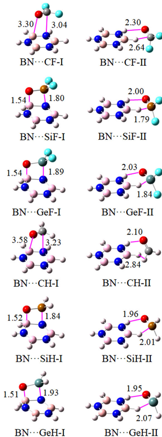
FIGURE 4 Optimized structures of the complexes pairing borazine with R_2TO , designated BN \cdots TH/TF ( T = C, Si, \text{ and } Ge ). Distances are in Å
