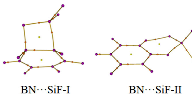
FIGURE 5 The atoms in molecules diagrams of BN...SiF-I and BN...SiF-II. Small dots refer to bond critical points
